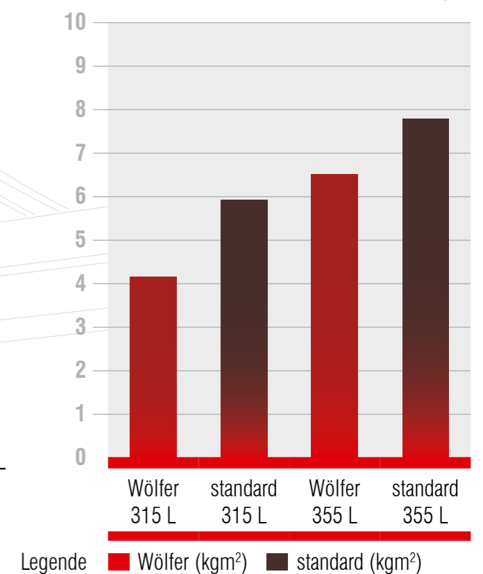
IP 55 400V-50Hz – moment of inertia (kgm 2 )
